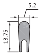
ALÜMİNYUM RAY ALUMINIUM RAIL
