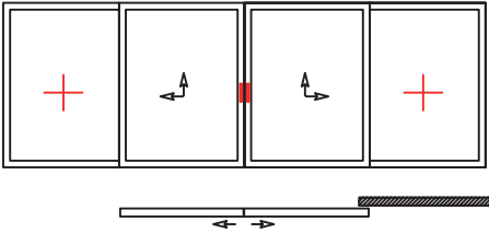
2 HAREKETLİ 2 SABİT KANAT 2 SLIDING 2 FIX SASH
