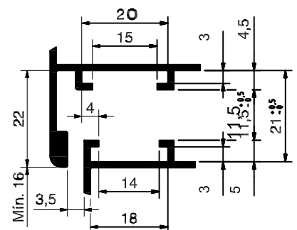
EUROGROOVE PROFILE
