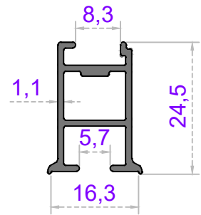
ARKA SABİT
